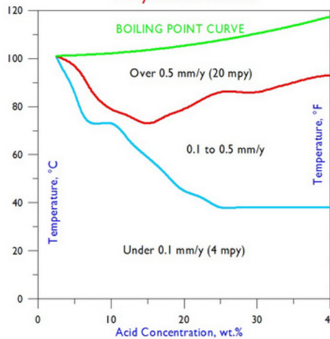
Iso-Corrosion Diagram for C-276 Alloy in Nitric Acid
